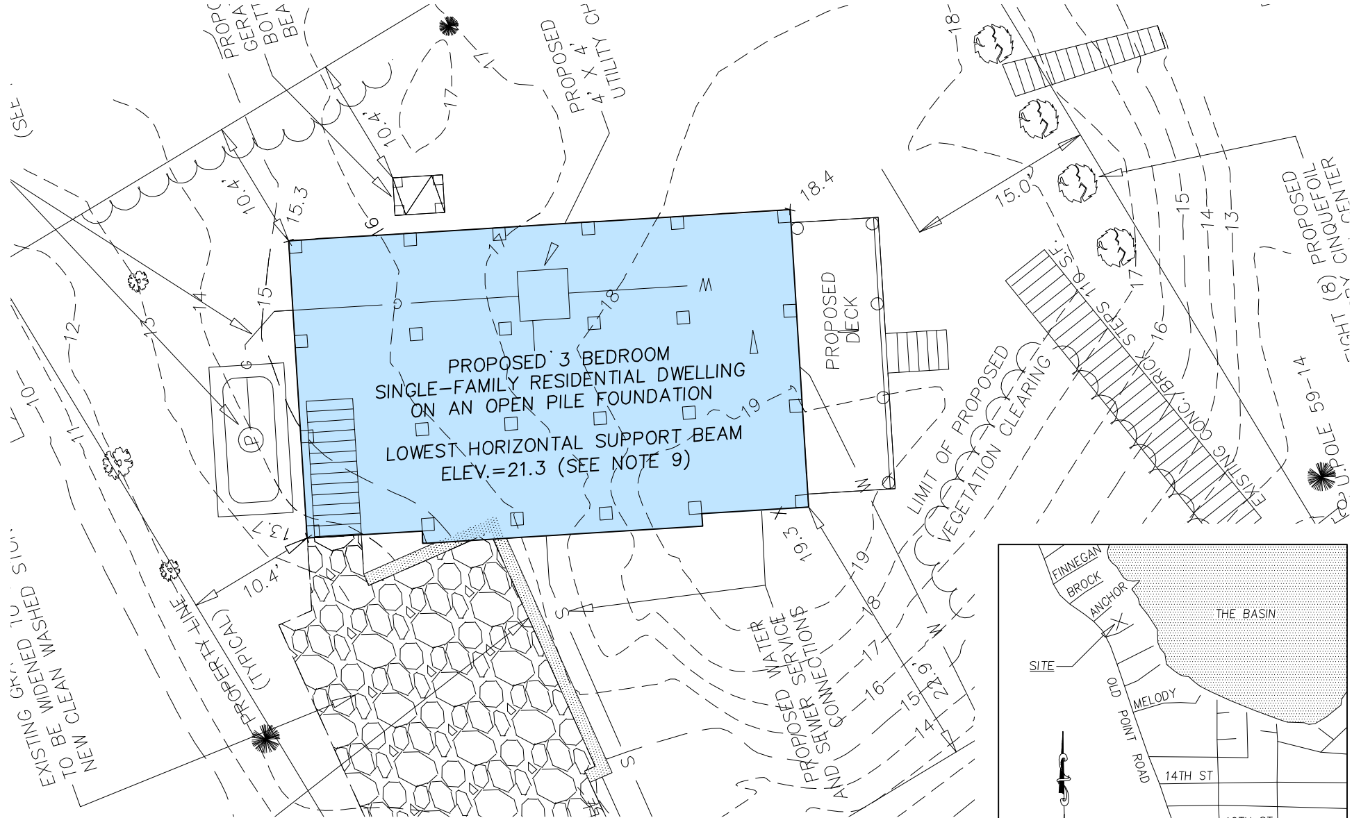
SITE PLAN
